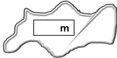
Depth of the ice in Antarctica
