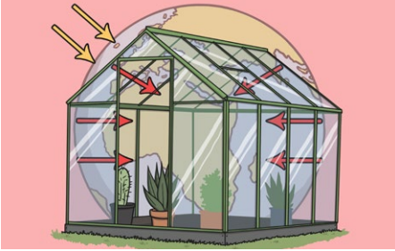
Greenhouse Gases
