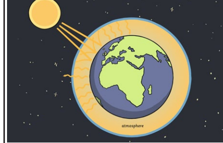
Global Warming
